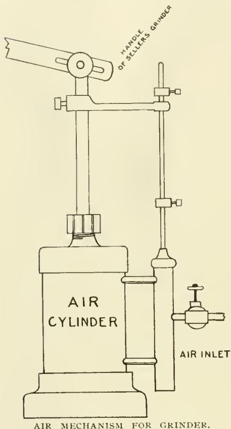
AIR MECHANISM FOR GRINDER.
